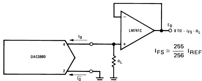
FIGURE 10. Negative Low Impedance Output Operation (Note 5)
