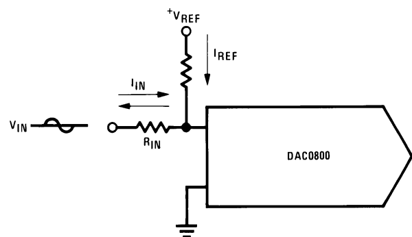
FIGURE 13. Accommodating Bipolar References (Note 5)
